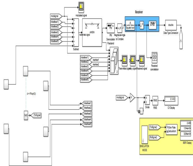
Figure 6. Matlab Model of the cellular Network
