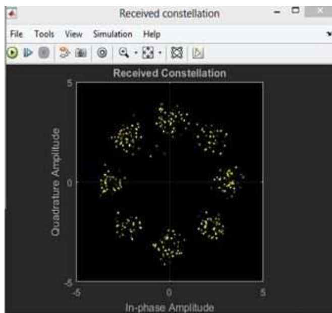
Figure 4.15. Received constellations for case 3 simulation
