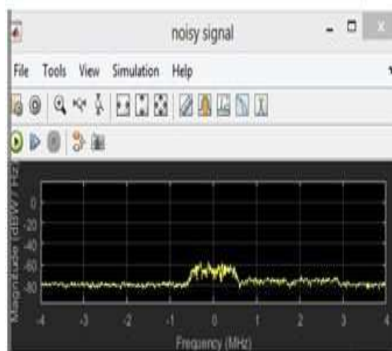
Figure 4.7.Noise signal for case 2 simulation
