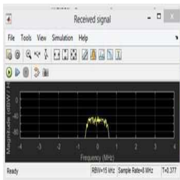
Figure 4.14.Received signal for simulation for case 3
