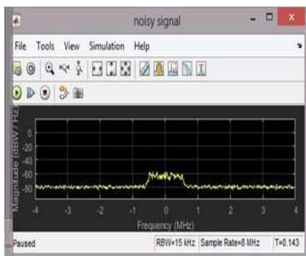
Figure 4.2.Noise signal for case 1
