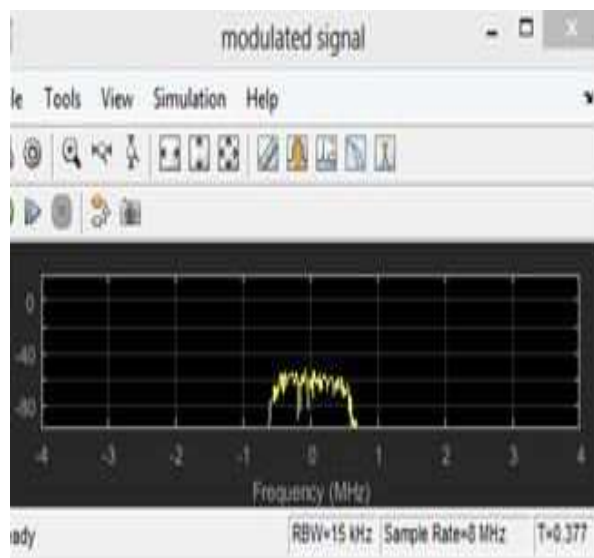
Figure 4.13.Modulated signal for simulation case 3
