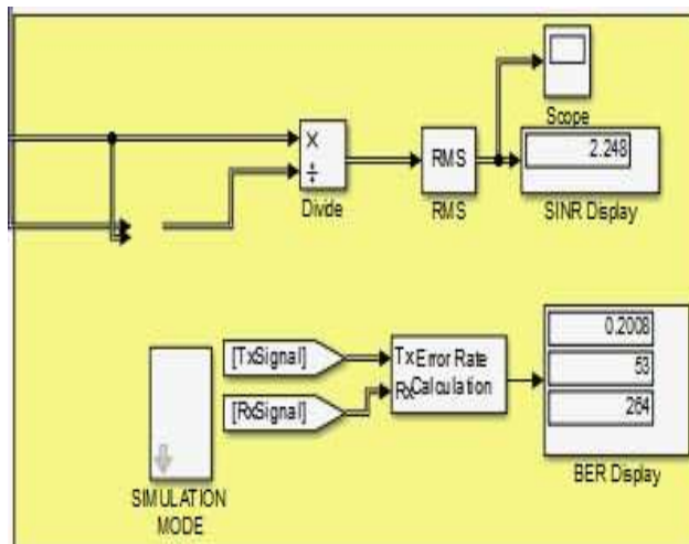
Figure 4.1.Result of Simulation case 1 showing S/I ratio and BER
