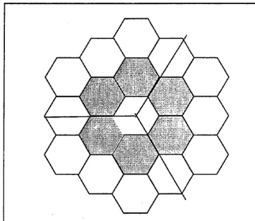
Figure 5.120 sectoring with the first (gray shaded) and second tier co-channel cells.
