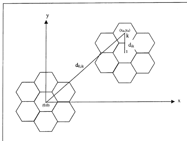
Figure 3. The coordinates of the reference base station and an interfering mobile station
