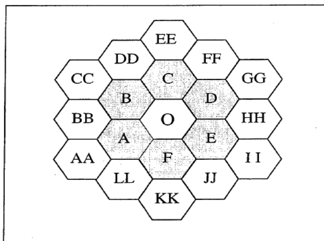
Figure 2. Reference cell with the first tier (gray shaded) and second tier co-channel cells
