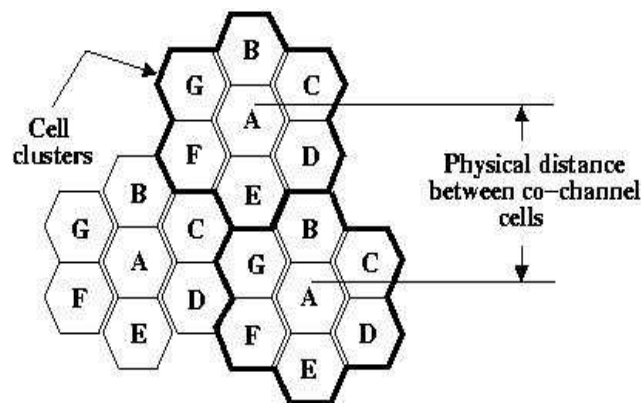
Figure 1. Schematic diagram of frequency reuse
