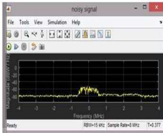
Figure 4.12.Noise signal for simulation case 3
