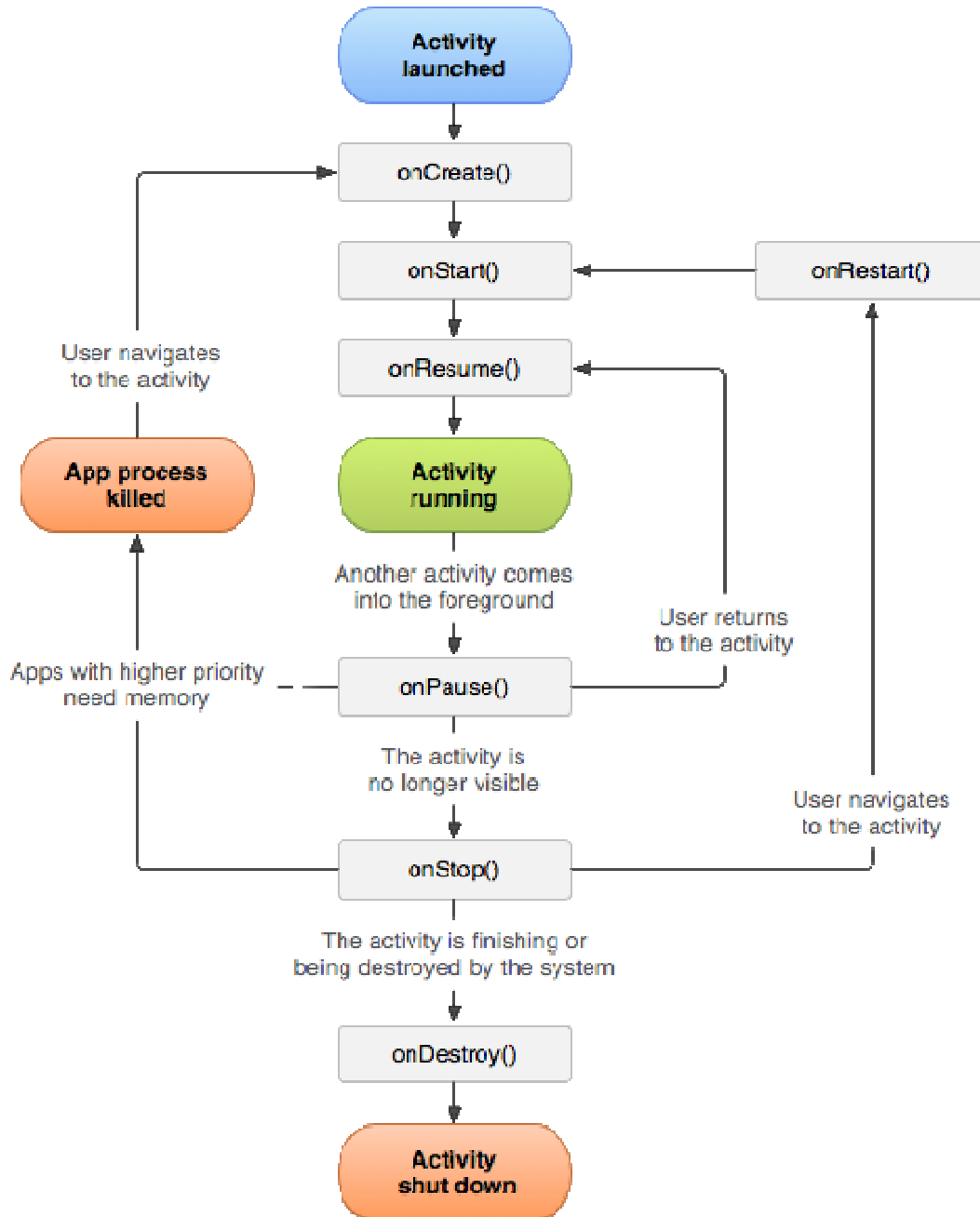
Figure 1.A simplified illustration of the activity lifecycle for basic android application
